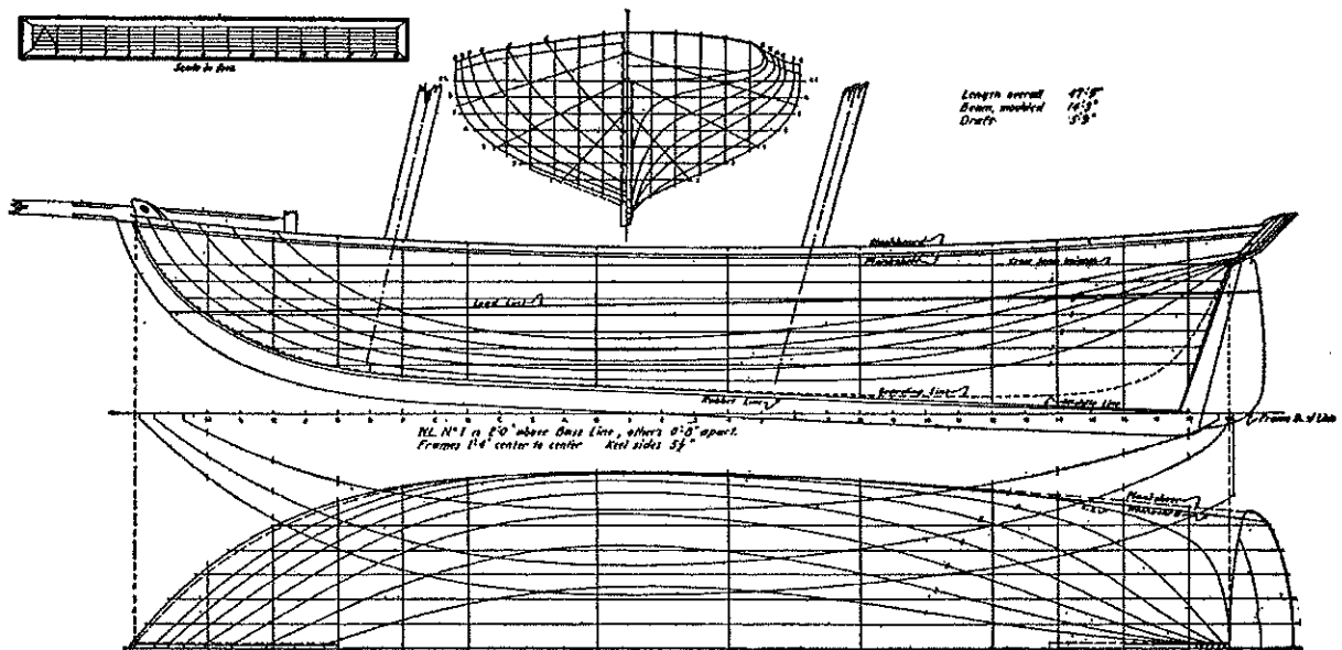
Lines of a schooner-yacht, the Dream, built at New York City, in 1833, by Isaac Webb; showing lines drawn to inside of planking, old-fashioned upper and lower transoms, flaring topsides, straight rise of floor, greatest beam forward of mid-length and straight keel. Ballast all inside. Sawn frames. Note that "cross seam" is the bottom of the lower transom at rabbet of post.
